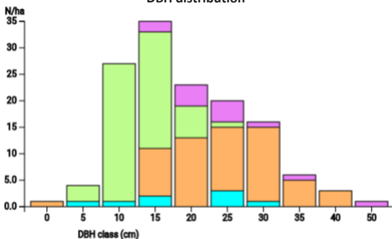
*DBH distribution
