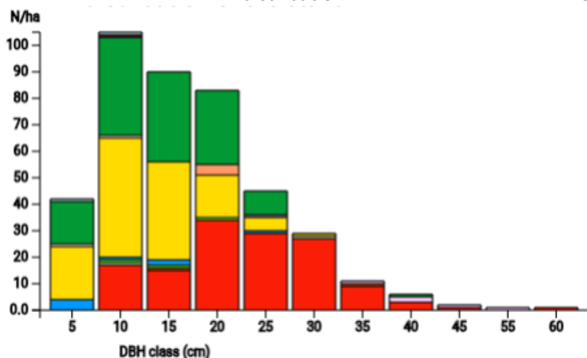
DBH distribution
