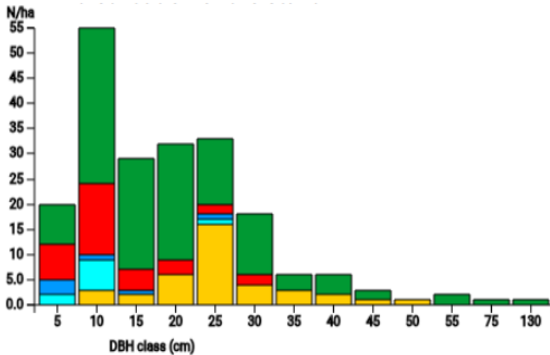
DBH distribution
