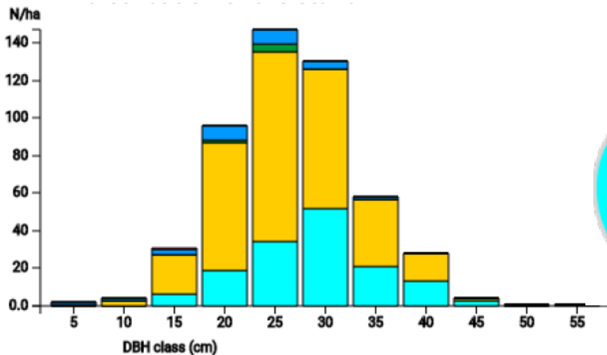
DBH distribution
