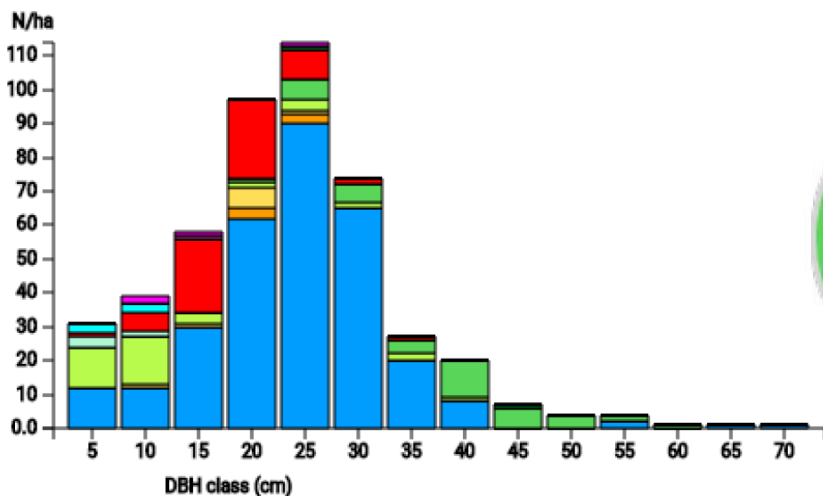
DBH distribution
