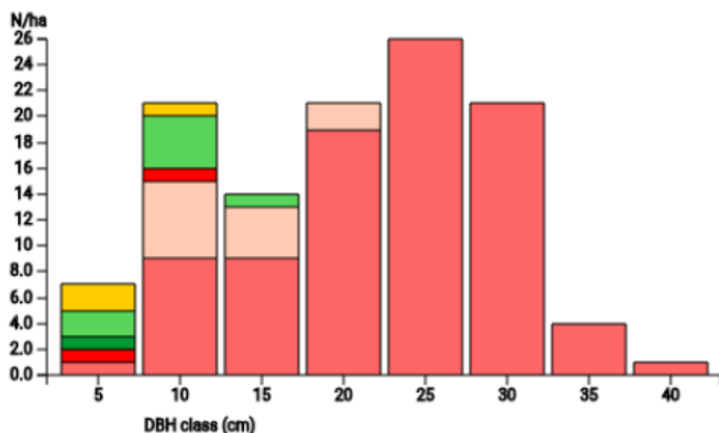
*DBH distribution
