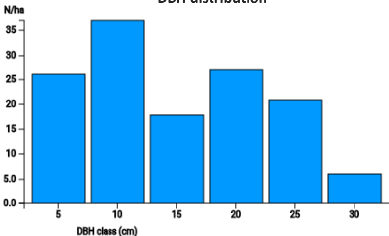
*DBH distribution
