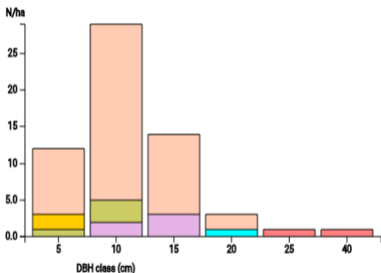
*DBH distribution
