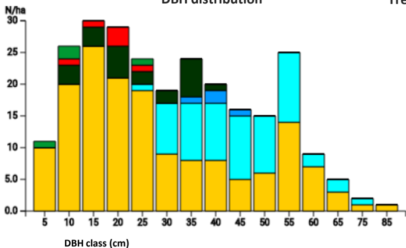
DBH distribution
