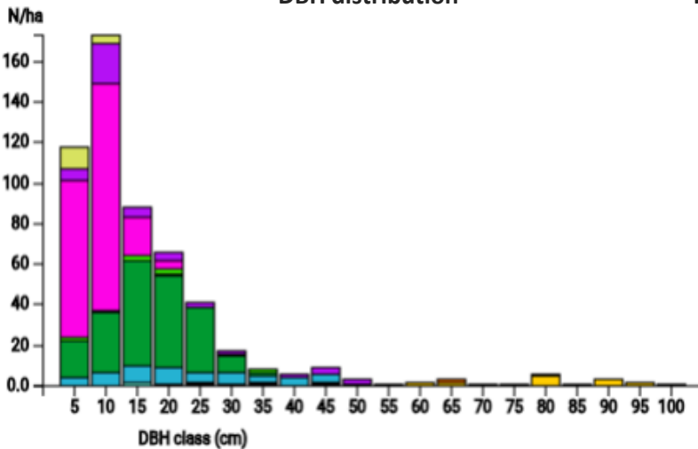
DBH distribution
