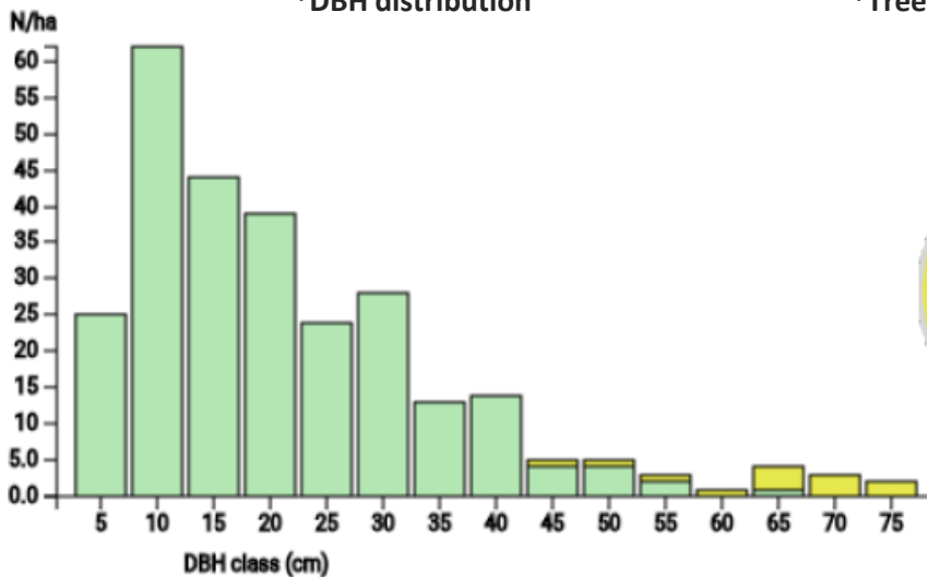
*DBH distribution
