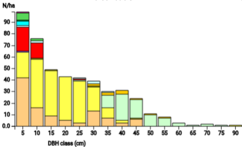
DBH distribution
