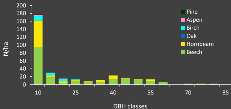
DBH distribution
