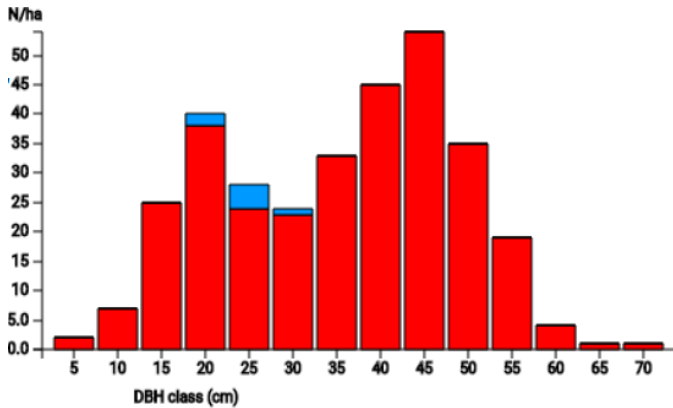
DBH distribution
