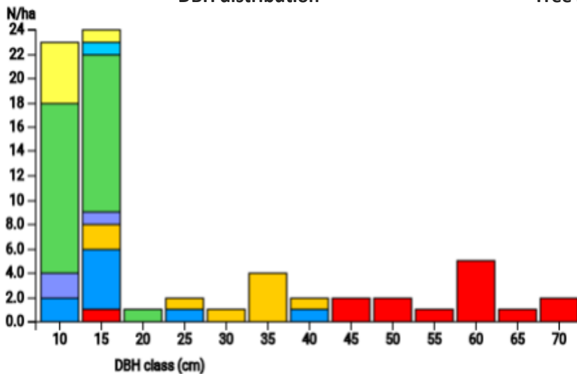
*DBH distribution
