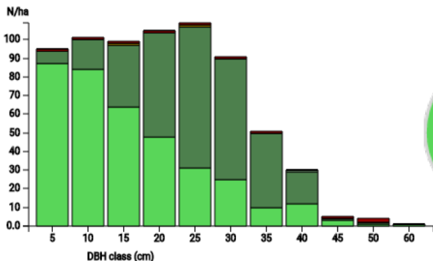
DBH distribution
